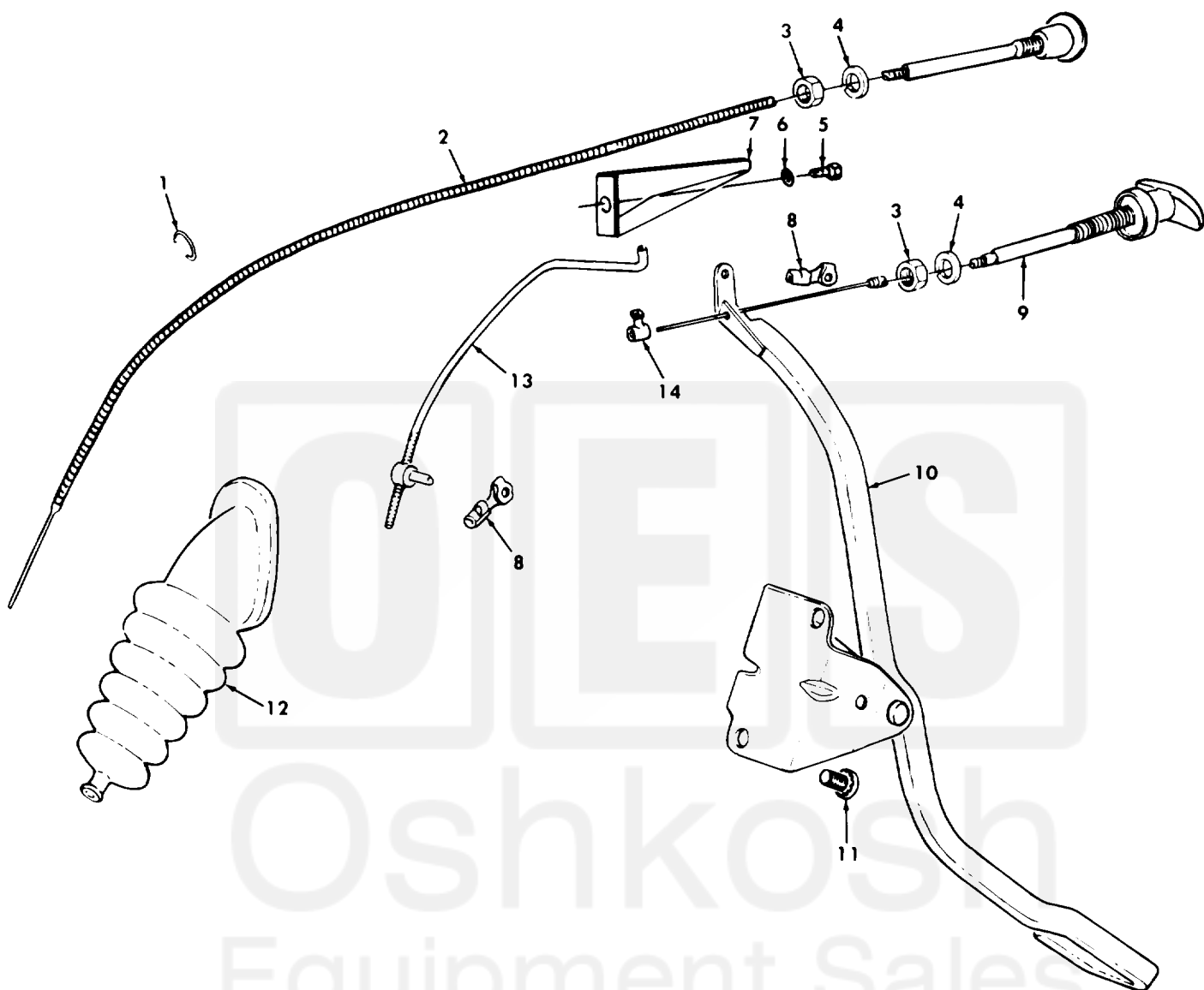
Figure 31. Accelerator, Throttle, and Choke Controls.
